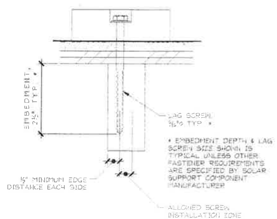
Figure 3. Typical Anchor with Lag Screw Attachment.
